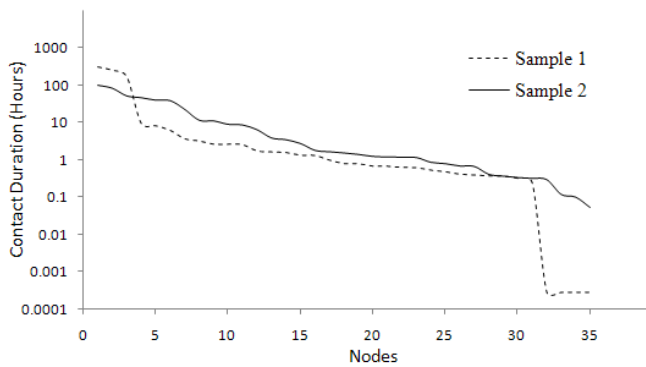
Figure 4. Contact duration between two sample participants and other nodes during the experiment
