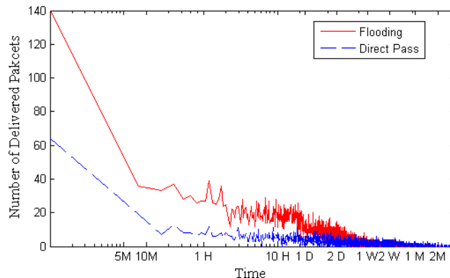
Figure 7. End-to-End delivery time histogram for Direct Pass and Flooding algorithms
